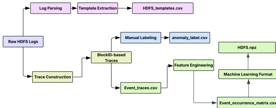
Figure 4.1: Preprocessing Pipeline
